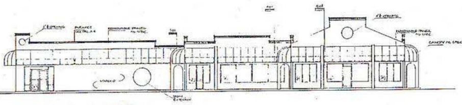
FRONT ELEVATION SCALE: 1/4"=1'-0"
